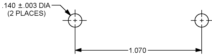
MOUNTING HOLE LAYOUT HORIZONTAL FLANGE MOUNT (HFM)
